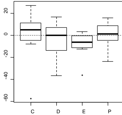
delta.Ki67
