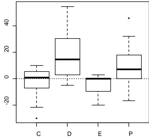
percent.tumor.change
