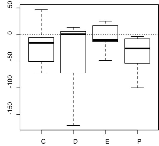
delta.pMET
