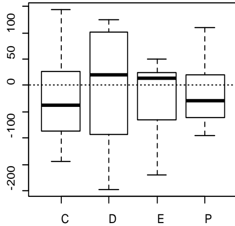
delta.Ecadherin
