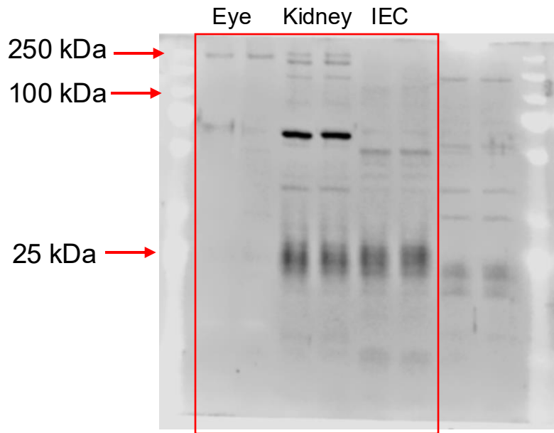
Crb3a blot
