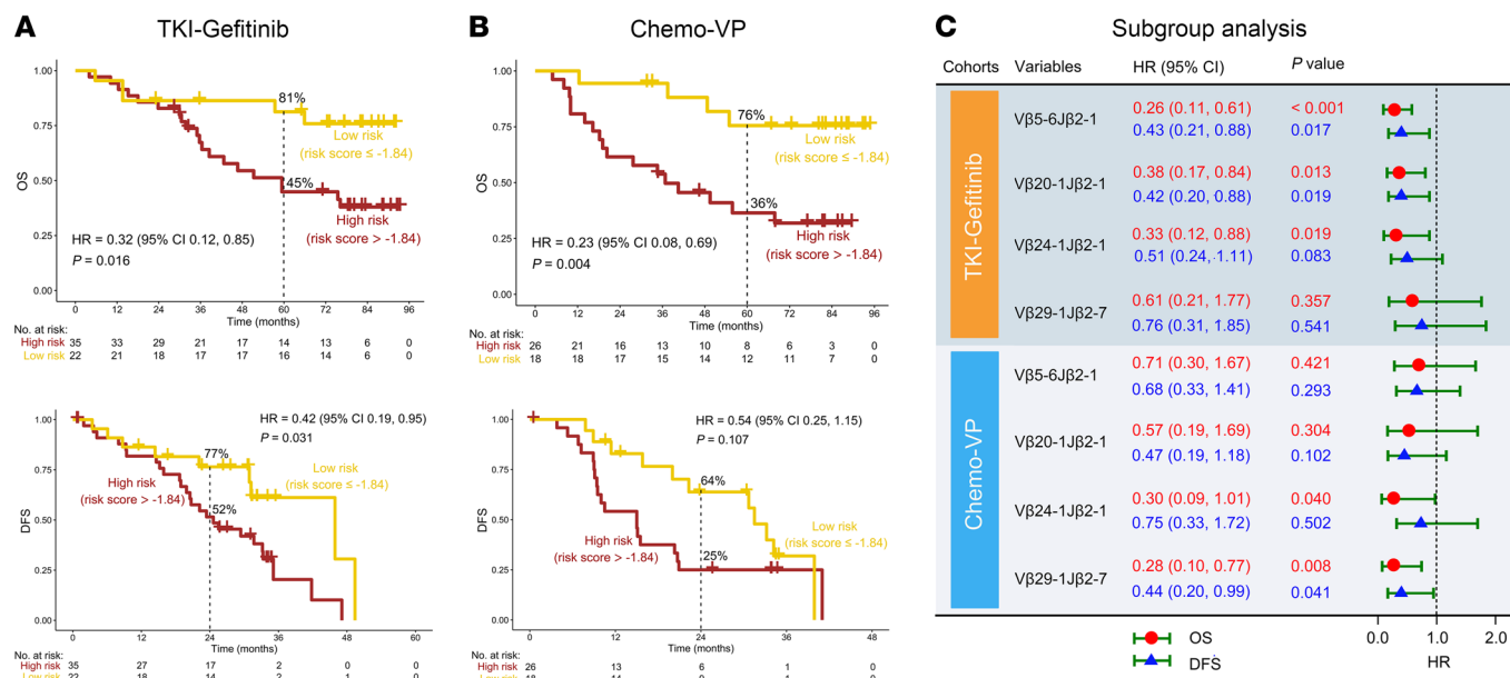
Figure 6. Kaplan-Meier survival analysis of TCRs in the TKI-gefitinib and Chemo-VP cohorts. A weighted combination of 4 TCRs for overall survival (OS) (top) and disease-free survival (DFS) (bottom) analysis in the TKI-gefitinib (A) and Chemo-VP (B) cohorts. (C) OS and DFS analysis of Vβ5-6Jβ2-1, Vβ20-1Jβ2-1, Vβ24-1Jβ2-1, and Vβ29-1Jβ2-7 by Kaplan-Meier analysis in the TKI-gefitinib and Chemo-VP cohorts.
