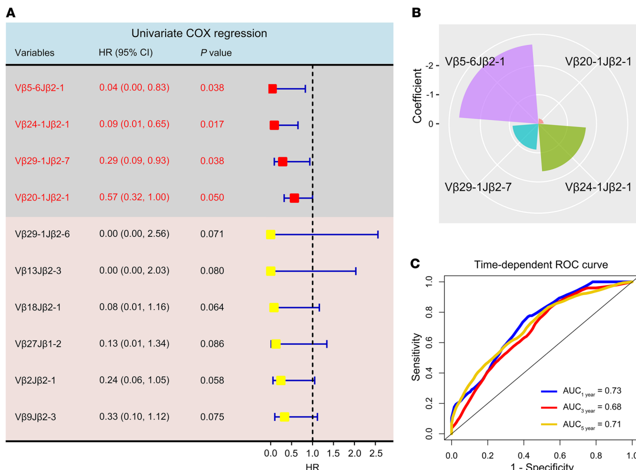
Figure 3. Uni- and multivariate COX regression analysis of differentially expressed TCRs. (A) Forest plot of univariate COX regression analysis showing that clonal TCRs are associated with favorable overall survival (OS) based on P < 0.1 . The statistically significant TCRs are shown in red, with a P \leq 0.050 . (B) The radar plot shows the contribution of the 4 TCRs to OS, which was determined by the coefficients of the 4 TCRs in the multivariate COX regression model. The smaller areas represent a lower contribution, whereas the larger areas represent a greater contribution. (C) A time-dependent receiver operating characteristic (ROC) curve plotted by the “survivalROC” package in R (version 4.0.2) was used to evaluate the performance of the multivariate COX regression model. AUC of more than 0.5 indicated that the model had better performance.
