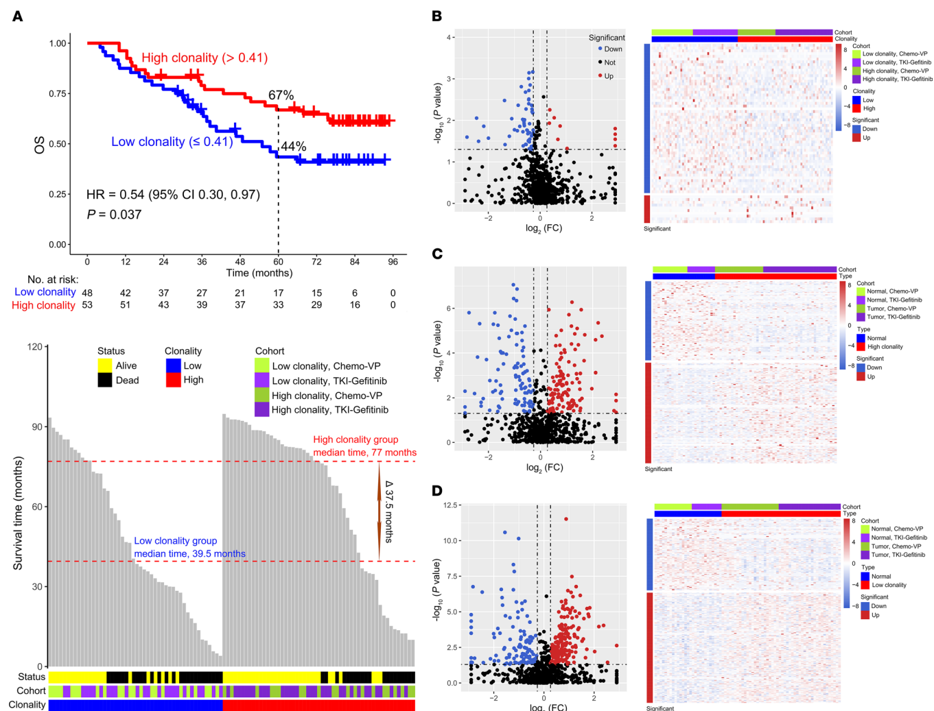
Figure 2. Overall survival analysis of patients with EGFR mutant lung cancer based on the clonality level. (A) Probability of overall survival (OS) for patients with high and low clonality (top). Distribution of the OS time of patients with low and high clonality (bottom). (B–D) Identification of differentially expressed TCRs by the Mann-Whitney-Wilcoxon test based on the high vs. low clonality groups (B), the high clonality group vs. tumor-adjacent tissue (C), and the low clonality group vs. tumor-adjacent tissue (D). Volcano plots show the differentially expressed TCRs between 2 groups (left). An absolute value of the fold change (FC) of more than 1.2 and a P value of less than 0.05 were used as a threshold to determine the significance of the differentially expressed TCRs. The red dots represent upregulated TCRs, the blue dots represent downregulated TCRs, and the black dots represent TCRs that did not change significantly. The heatmap shows the frequency of the differentially expressed TCRs based on an absolute value of fold change of more than 1.2 and a P value of less than 0.05 between 2 groups (right).
