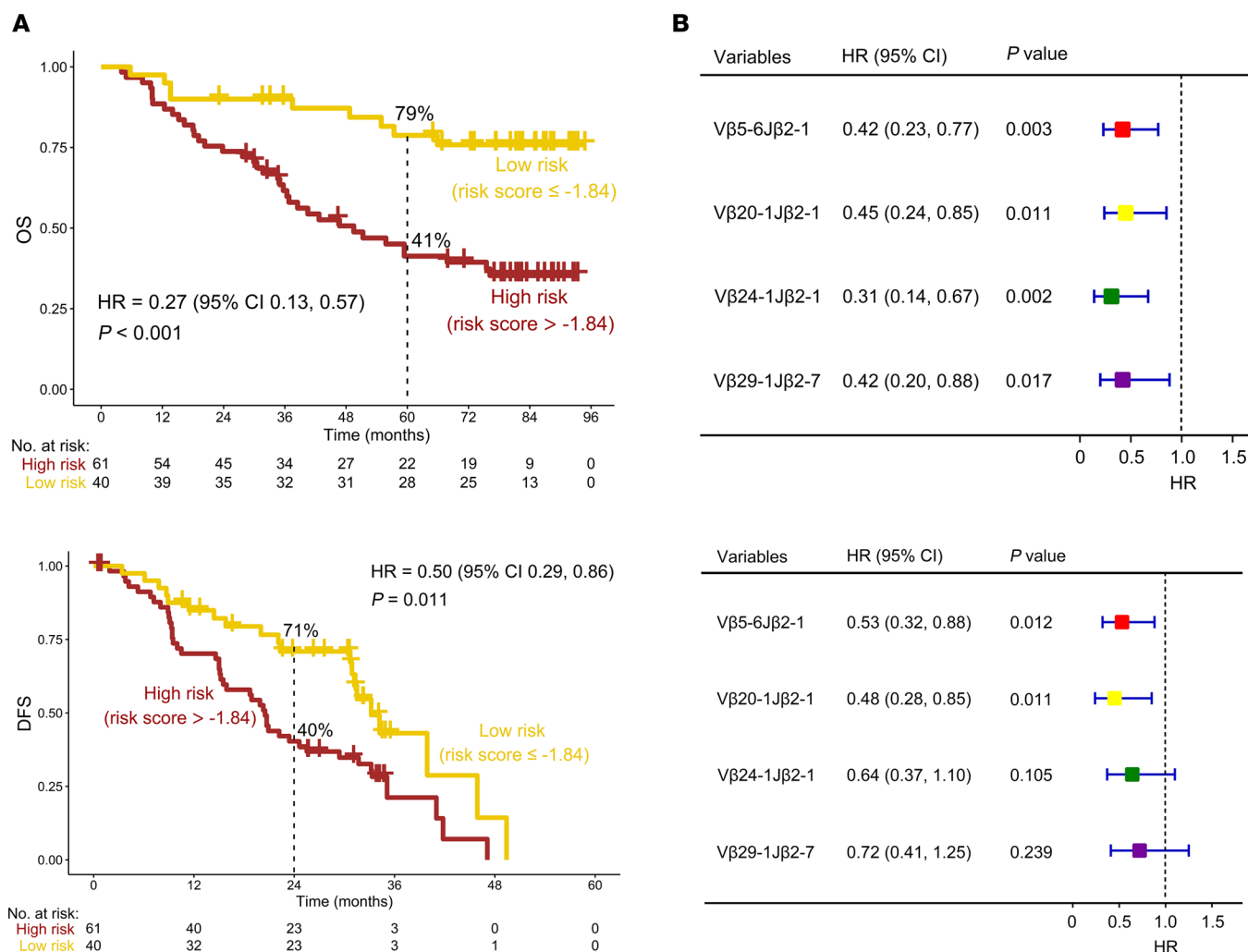
Figure 4. A weighted combination of 4 TCRs was associated with the prognosis of patients with an EGFR mutation with NSCLC. (A) Overall survival (OS) (top) and disease-free survival (DFS) (bottom) analysis of low- and high-risk patients based on the combination of 4 TCRs. (B) OS (top) and DFS (bottom) analysis of patients with a low and high frequency of V \beta 5-6J \beta 2-1, V \beta 20-1J \beta 2-1, V \beta 24-1J \beta 2-1, and V \beta 29-1J \beta 2-7 by Kaplan-Meier analysis.
