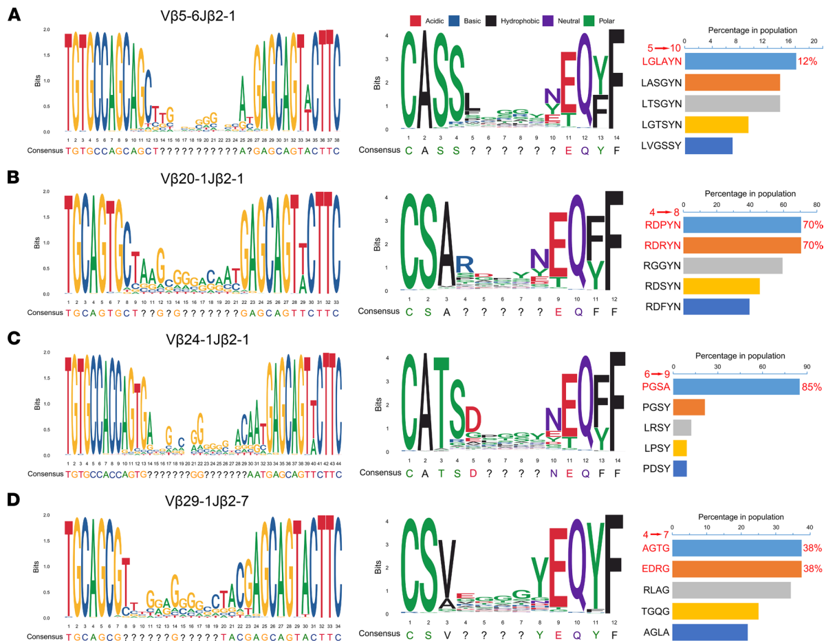
Figure 5. Sequence motif analysis of high-frequency groups of TCRs. Local alignment was used to calculate the similarity of the base (left) and amino acid (middle) sequences of Vβ5-6Jβ2-1 (A), Vβ20-1Jβ2-1 (B), Vβ24-1Jβ2-1 (C), and Vβ29-1Jβ2-7 (D), which were identified by the “msa” package and plotted by the “ggplot2” and “ggseqlogo” packages in R. The question marks indicate that the sequence at that position is not conservative. The proportion of the top 5 nonconservative amino acid sequences in patients with a high frequency of TCRs is also shown (right).
