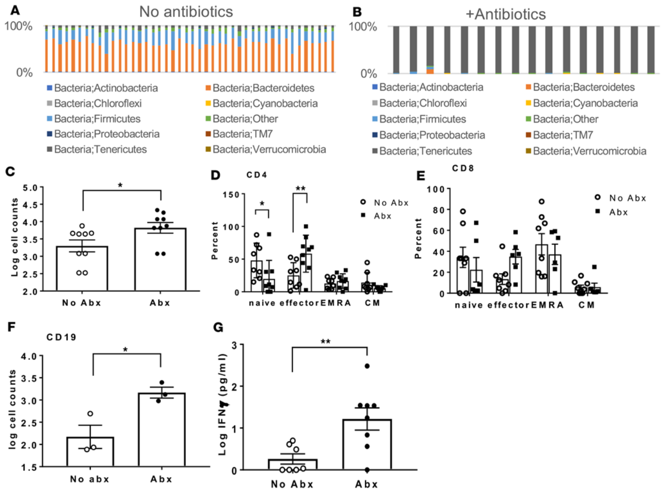
Figure 1. Changes in microbiota and lymphocytes with antibiotics. 16S sequencing was performed on freshly isolated pellets from humanized mice (A) and humanized mice treated with the cocktail of 4 antibiotics for 2 weeks (B). Following antibiotic treatment there was a 24 \pm 4.32 -fold depletion of Eubacteria ( n = 11, P = 0.0002 ) and a 34.7 \pm 1.86 -fold depletion of segmented filamentous bacteria ( P = 4.33 \times 10^{-9} ). The flora was largely restricted to Terrificutes spp. after antibiotic treatment. (C) The number of CD2 + cells in the lamina propria of the mice treated with antibiotics (Abx) compared with mice that did not receive antibiotics is shown (each symbol represents an individual mouse, P = 0.0382 , Student's t test). (D) There was a significant interaction between antibiotic treatment and CD4 + T cell subsets in the gut ( P = 0.0004 , 2-way ANOVA). Naive and effector T cells were decreased and increased, respectively. *P < 0.05 , **P < 0.01 ; n = 8 and 9 /group. (E) Similar findings were seen within the CD8 + T cells but the differences were not statistically significant. (F) The number of CD19 + cells in the lamina propria of the mice treated with antibiotics compared with mice that did not receive antibiotics is shown (each symbol represents an individual mouse; P = 0.0261 , Student's t test) (G) The circulating levels of IFN- \gamma were elevated in the antibiotic-treated mice. Each symbol represents an individual mouse that was or was not treated with antibiotics. **P = 0.008 , Student's t test. CM, central memory T cell; EMRA, effector memory RA T cell.
