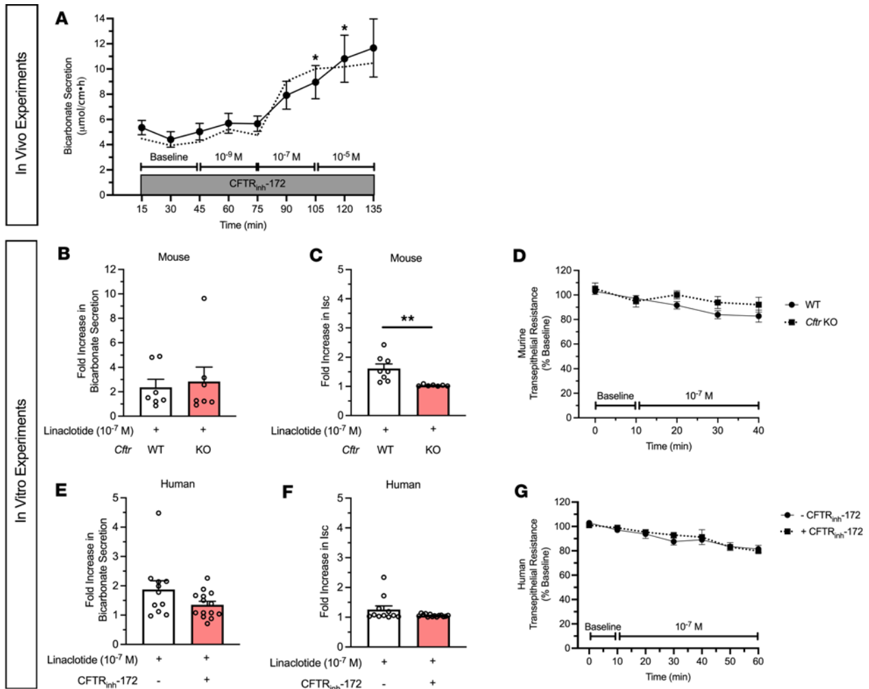
Figure 2. Linaclootide stimulates duodenal bicarbonate secretion independent of CFTR. (A) In vivo measurement of duodenal bicarbonate secretion in mice, similar to Figure 1A, with the exception that each perfusate also contained CFTR inh -172 ( 2 \times 10^{-5} M) ( n = 12 ). Dotted line is the mean response without CFTR inh -172 (from Figure 1A). * P < 0.05 vs. baseline by 1-way ANOVA. (B and C) In vitro duodenal mucosal bicarbonate secretion (B) and I_{sc} (C) in wild-type (WT) and Cfr -KO mice. Data are expressed as fold increase in linaclootide-stimulated responses over baseline bicarbonate secretion or I_{sc} in the same mouse. Each point ( n = 7 ) is a separate piece of duodenum from 5 mice. ** P < 0.01 by unpaired 2-tailed Student's t test. (D) Transepithelial resistance measurements in WT and Cfr -KO mice. (E–G) In vitro duodenal mucosal bicarbonate secretion (E), I_{sc} (F), and transepithelial resistance (G) in human endoscopic biopsies with or without CFTR inh -172 pretreatment ( 2 \times 10^{-5} M, 40–60 minutes). Each point ( n = 11 –14) represents a different biopsy. All data are means \pm SEM.
